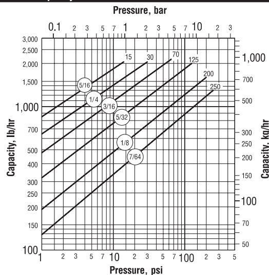
Model 22-DC Capacity
