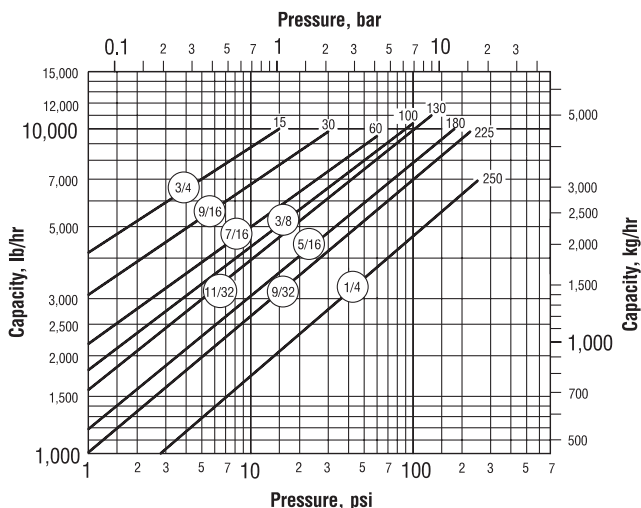
Model 25-DC Capacity
