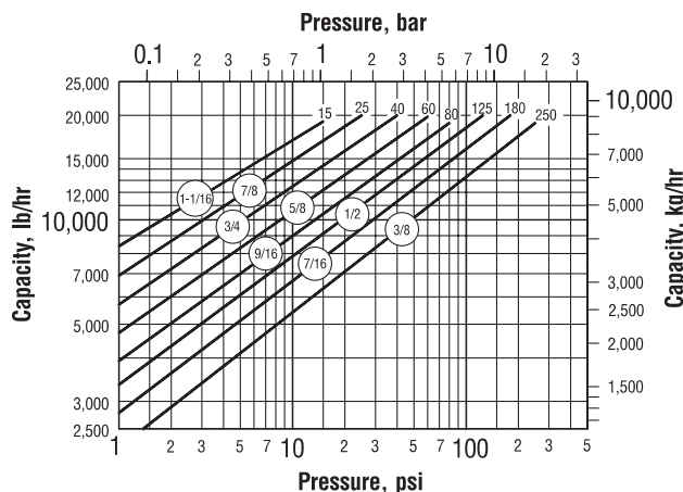
Model 26-DC Capacity
